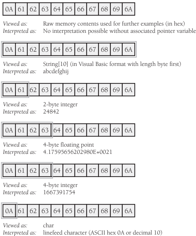
Figure 13-1 The amount of memory used by each data type is shown by double lines.
