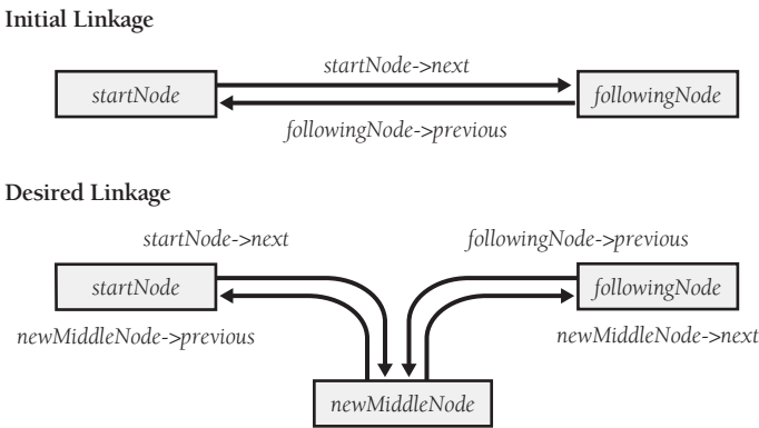
Figure 13-2 An example of a picture that helps us think through the steps involved in relinking pointers.
