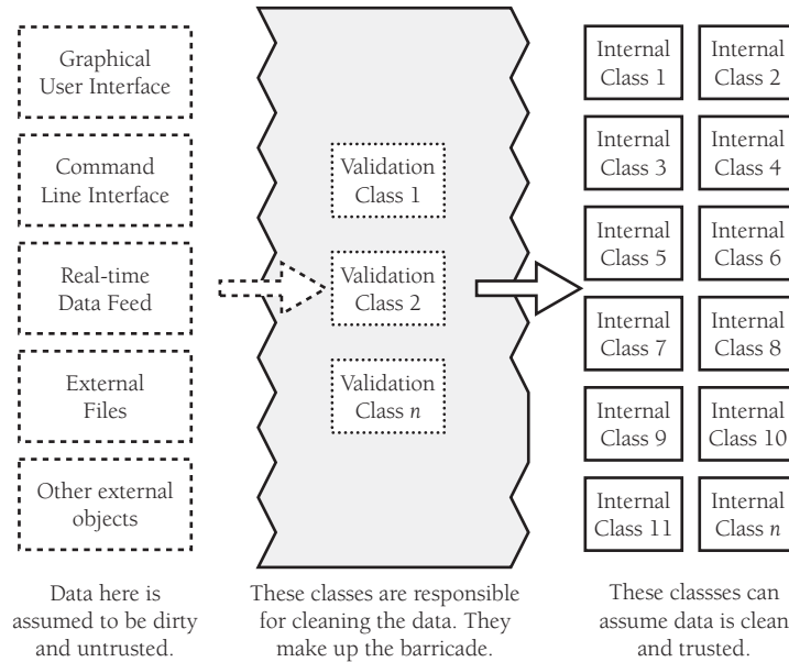
Figure 8-2 Defining some parts of the software that work with dirty data and some that work with clean data can be an effective way to relieve the majority of the code of the responsibility for checking for bad data.
